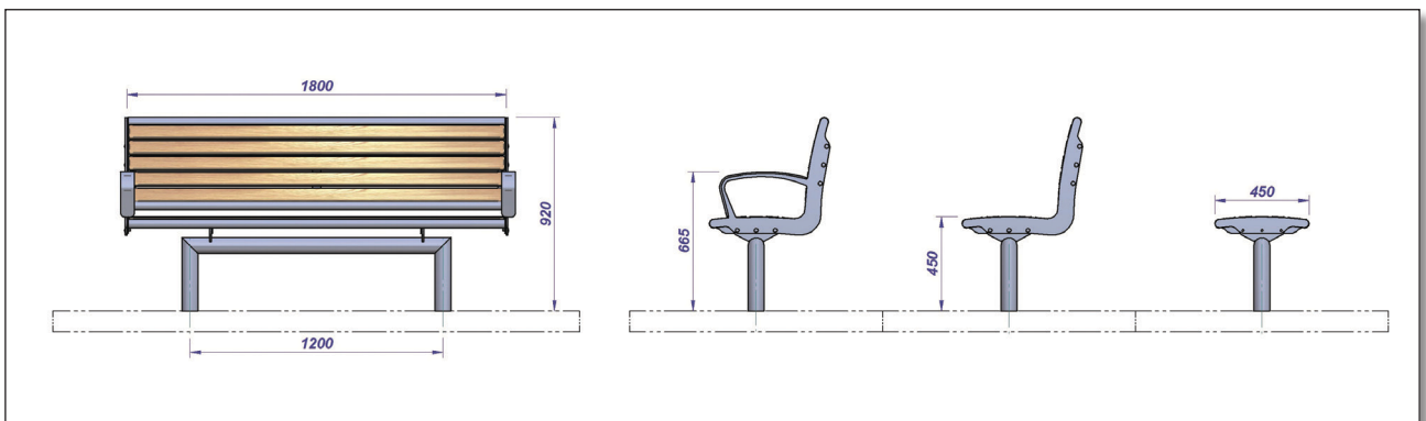
MODULAR DESIGN ALLOWS NUMEROUS CONFIGURATIONS
